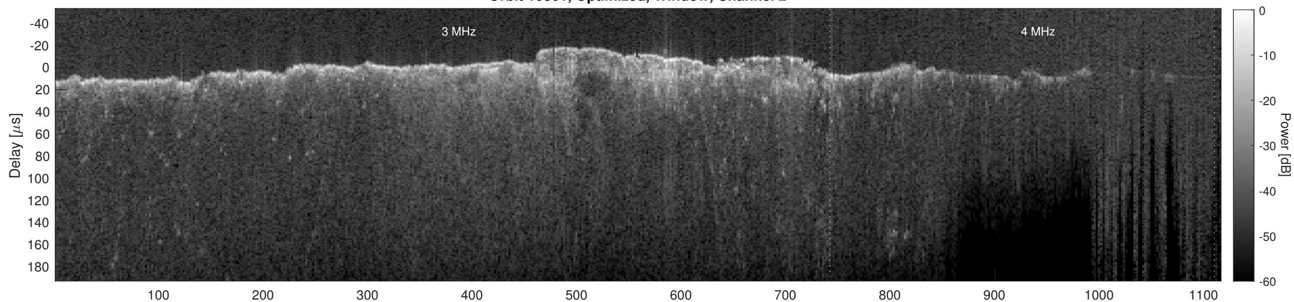
Orbit 10801, Cluttergram
