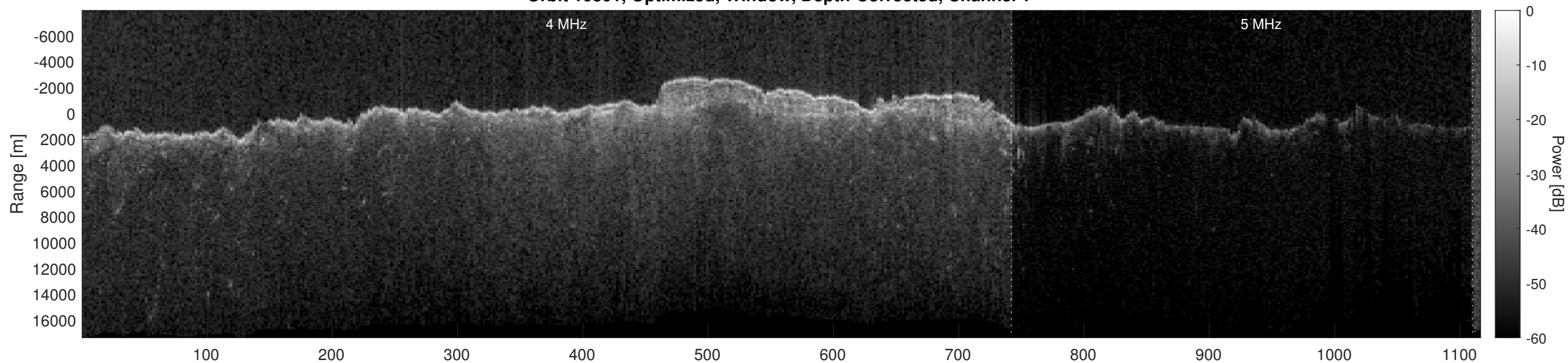
Orbit 10801, Optimized, Window, Depth-Corrected, Channel 2
