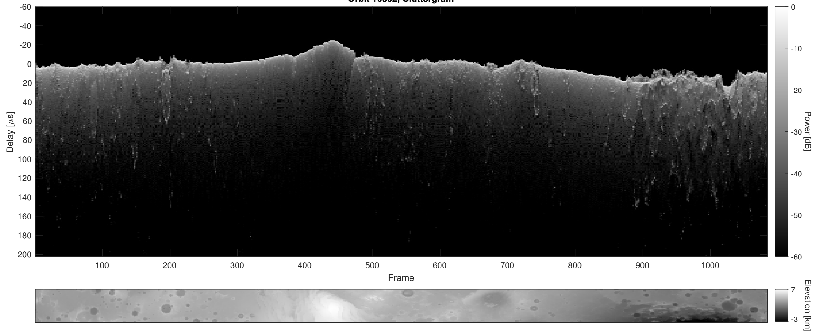
Orbit 10802, Cluttergram
