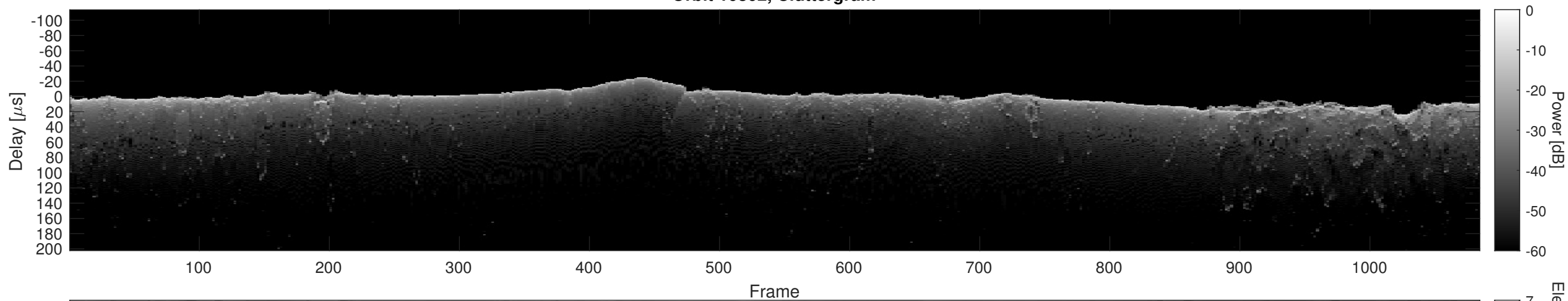
Orbit 10802, Cluttergram
