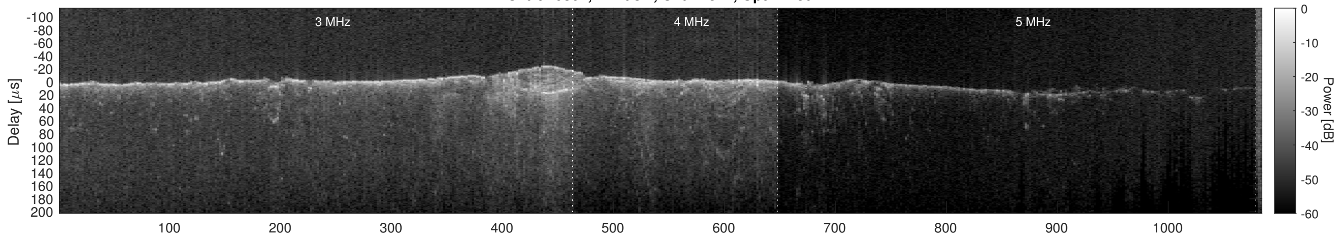
Orbit 10802, Cluttergram
