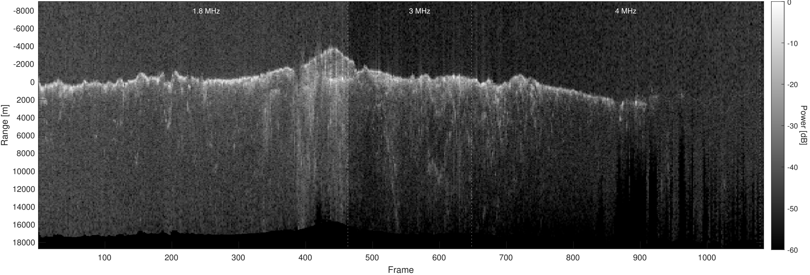
Orbit 10802, Optimized, Window, Depth-Corrected, Channel 2
