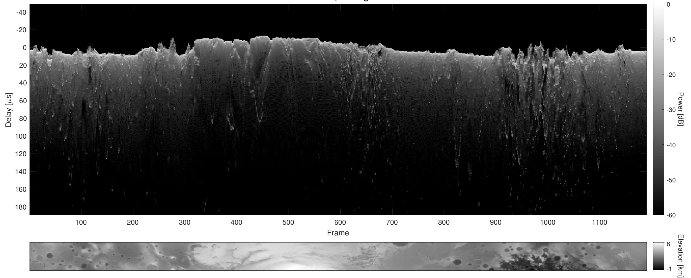
Orbit 10803, Cluttergram
