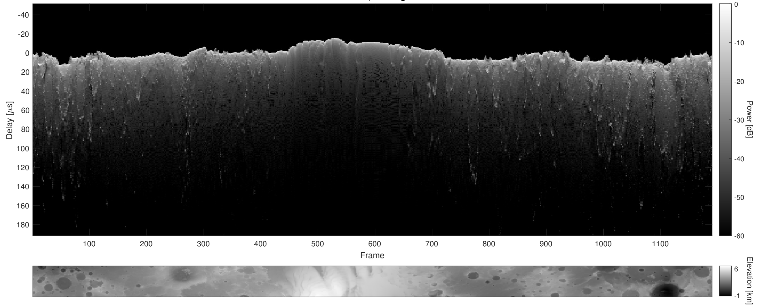
Orbit 10804, Cluttergram
