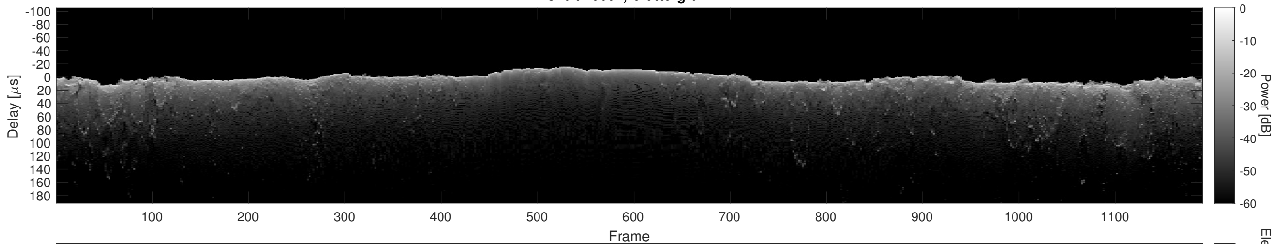
Orbit 10804, Cluttergram
