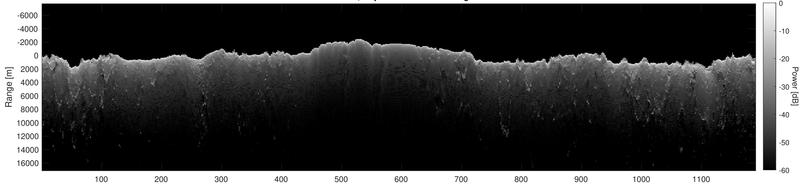
Orbit 10804, Depth-Corrected Cluttergram
