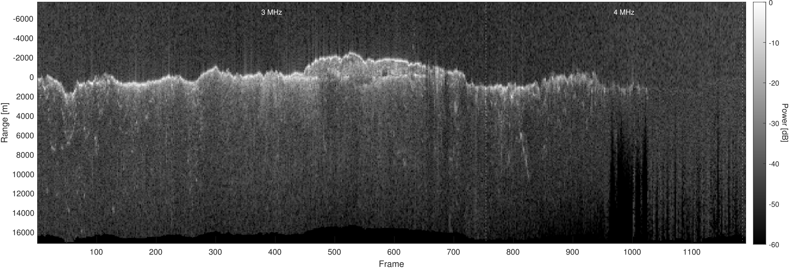
Orbit 10804, Optimized, Window, Depth-Corrected, Channel 2
