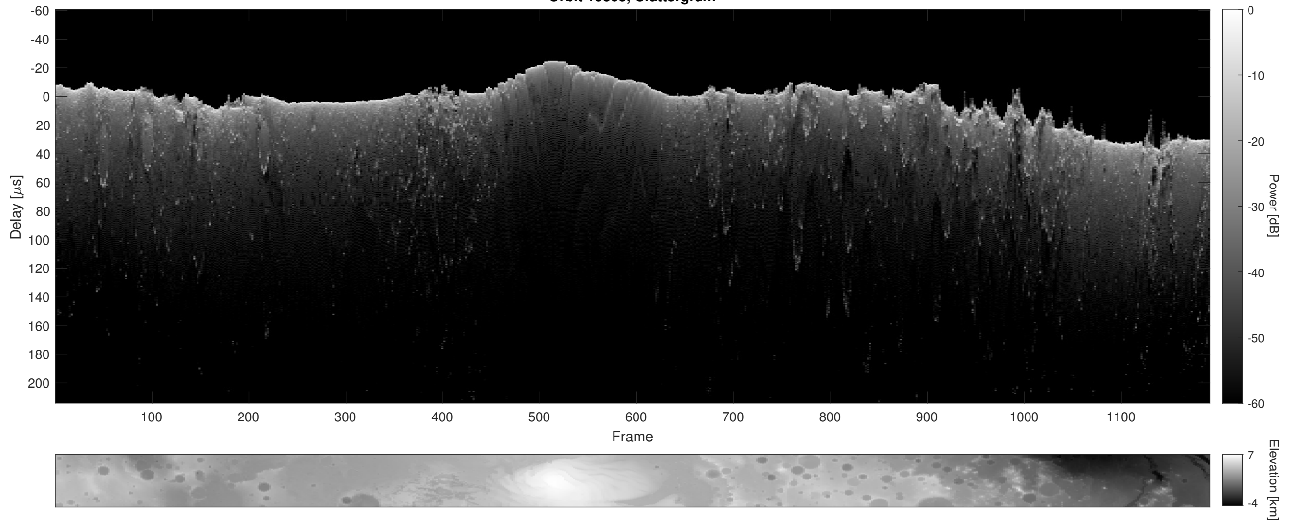
Orbit 10805, Cluttergram
