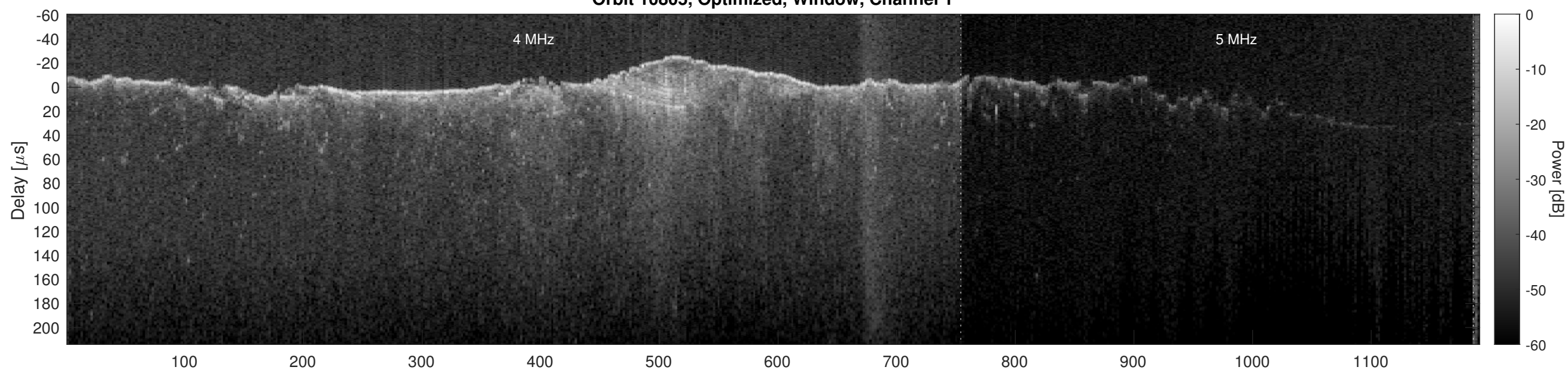
Orbit 10805, Optimized, Window, Channel 2
