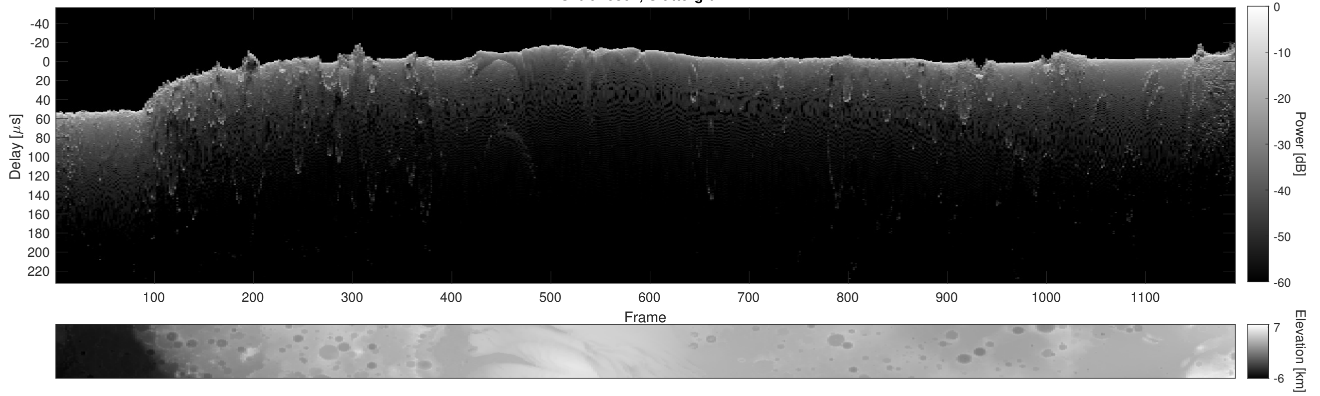
Orbit 10807, Cluttergram
