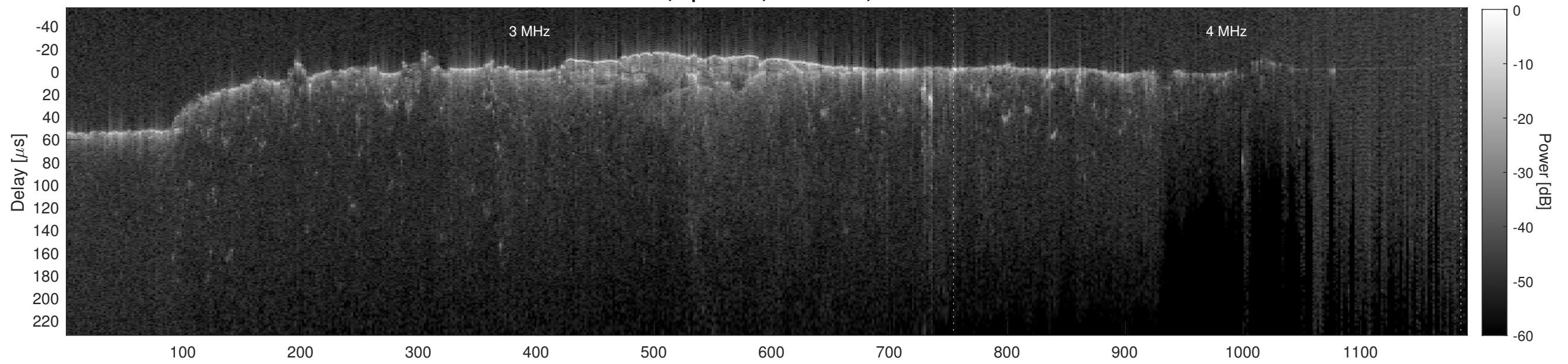
Orbit 10807, Cluttergram
