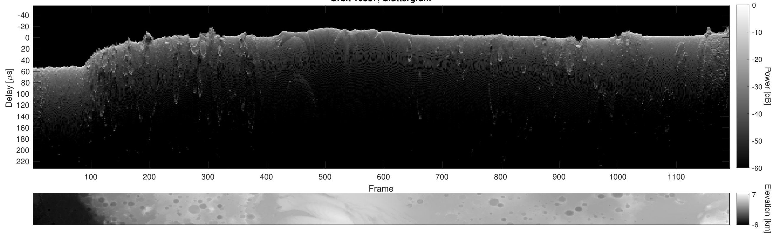
Orbit 10807, Cluttergram
