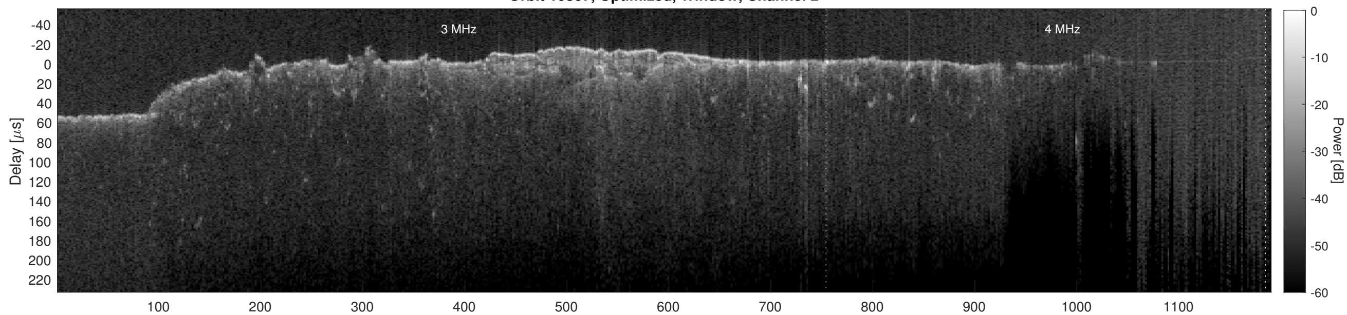
Orbit 10807, Cluttergram
