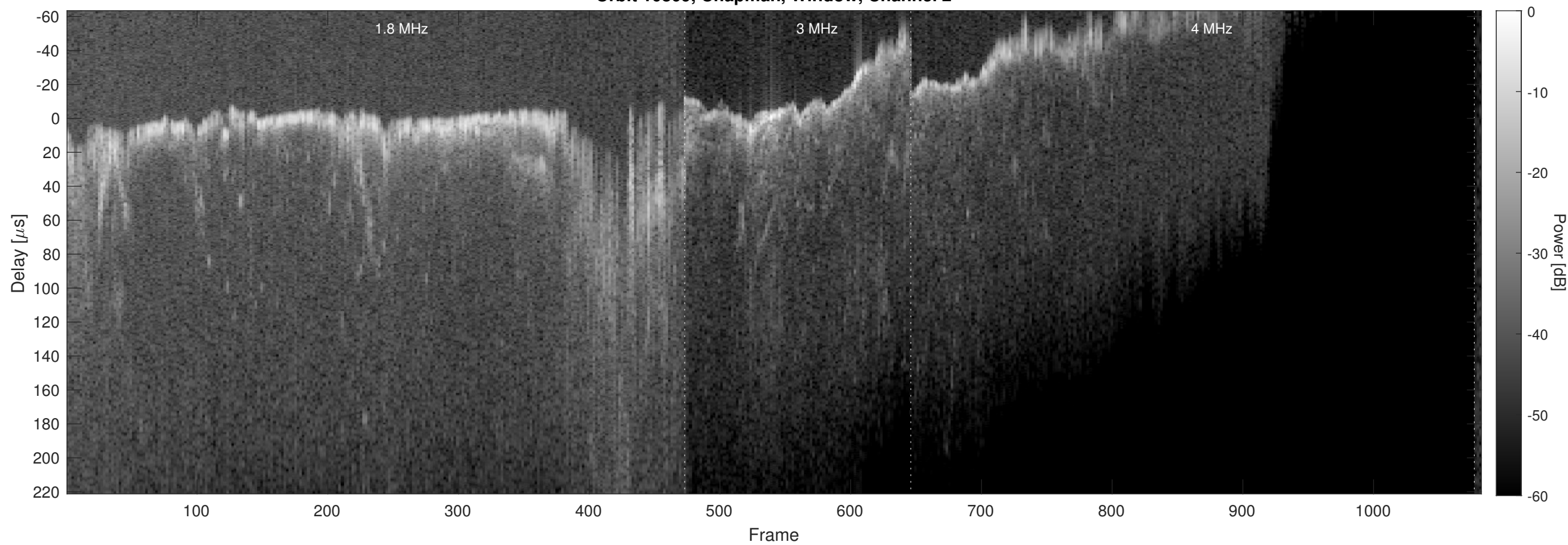
Orbit 10809, Chapman, Window, Channel 2
