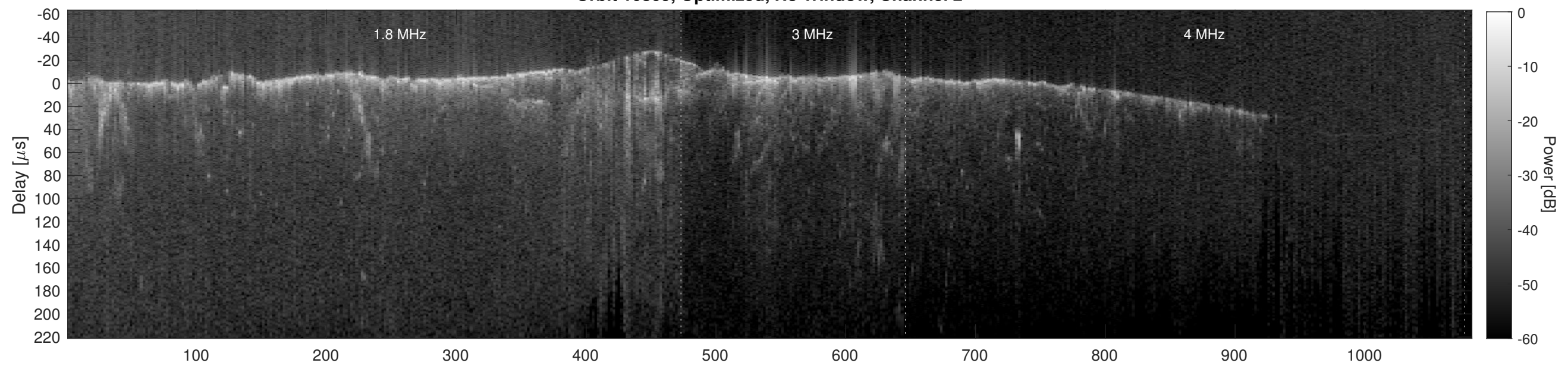
Orbit 10809, Cluttergram
