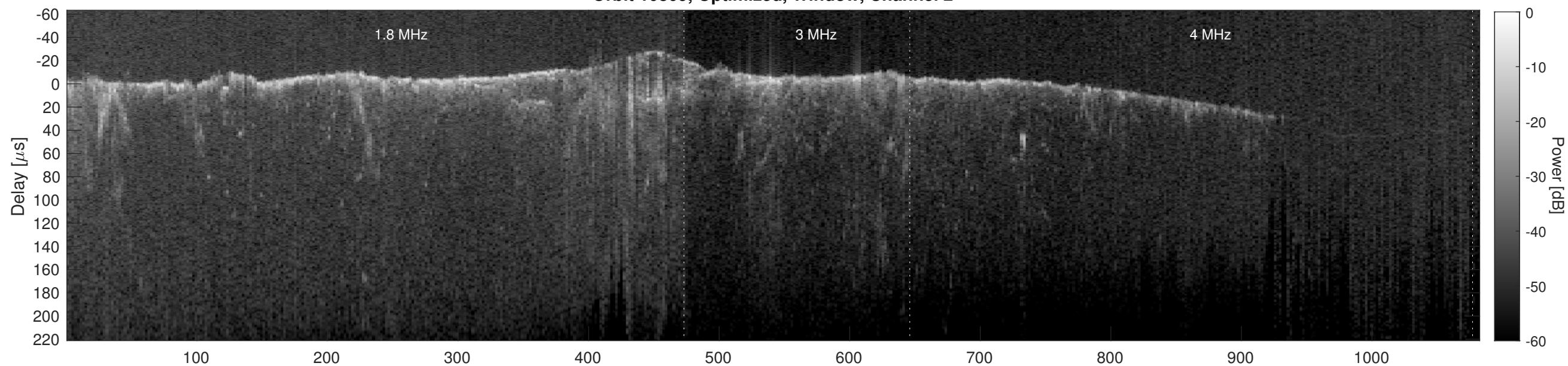
Orbit 10809, Cluttergram
