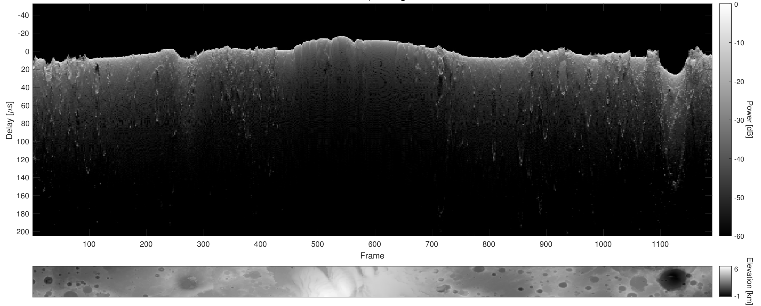
Orbit 10811, Cluttergram
