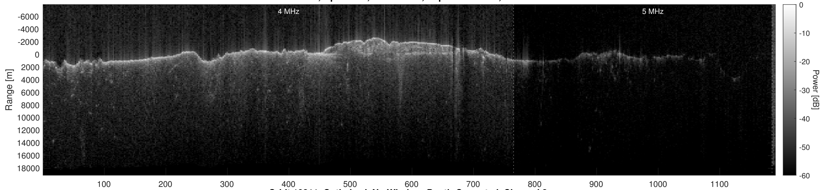
Orbit 10811, Optimized, No Window, Depth-Corrected, Channel 2
