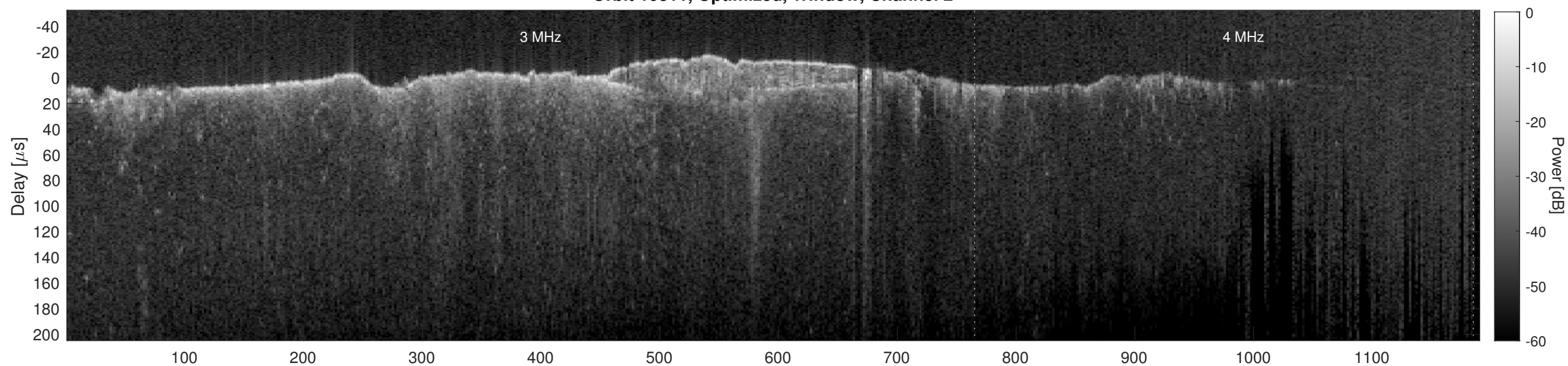
Orbit 10811, Cluttergram
