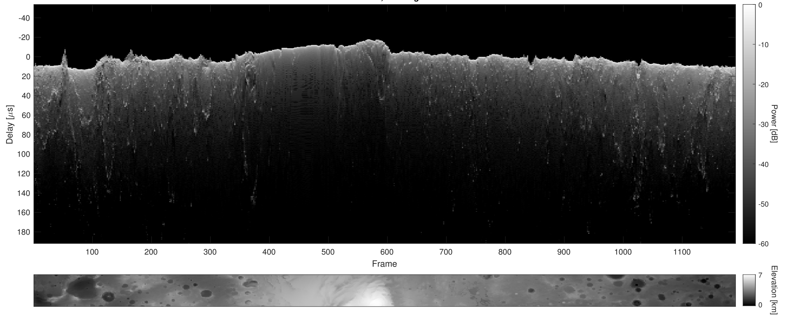
Orbit 10813, Cluttergram
