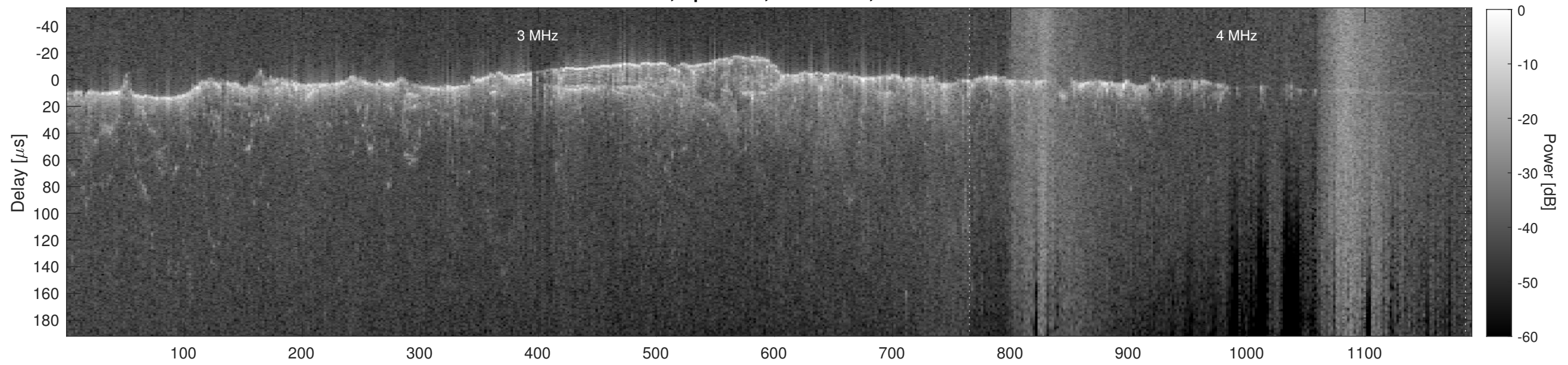
Orbit 10813, Cluttergram
