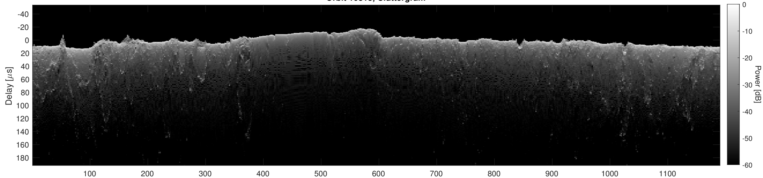
Orbit 10813, Cluttergram
