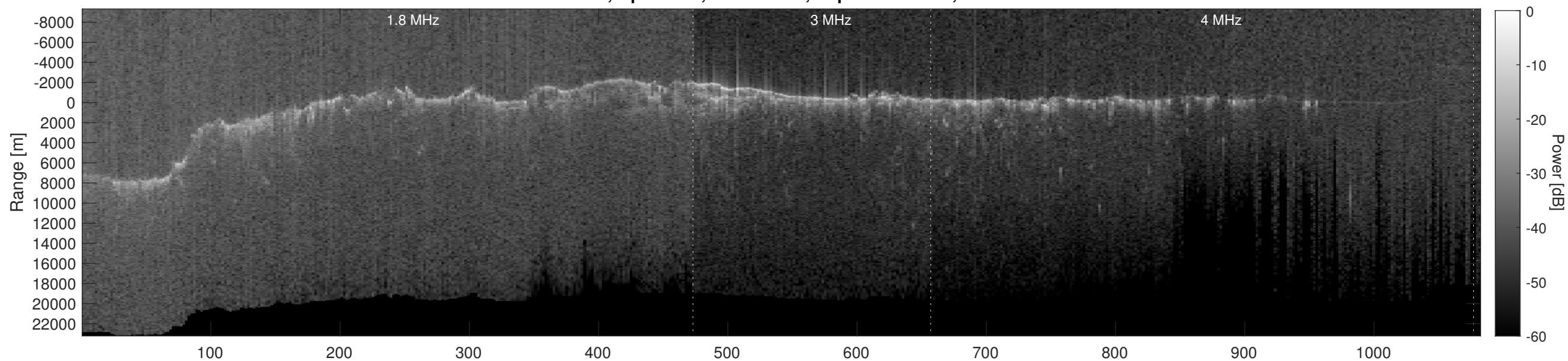
Orbit 10814, Depth-Corrected Cluttergram
