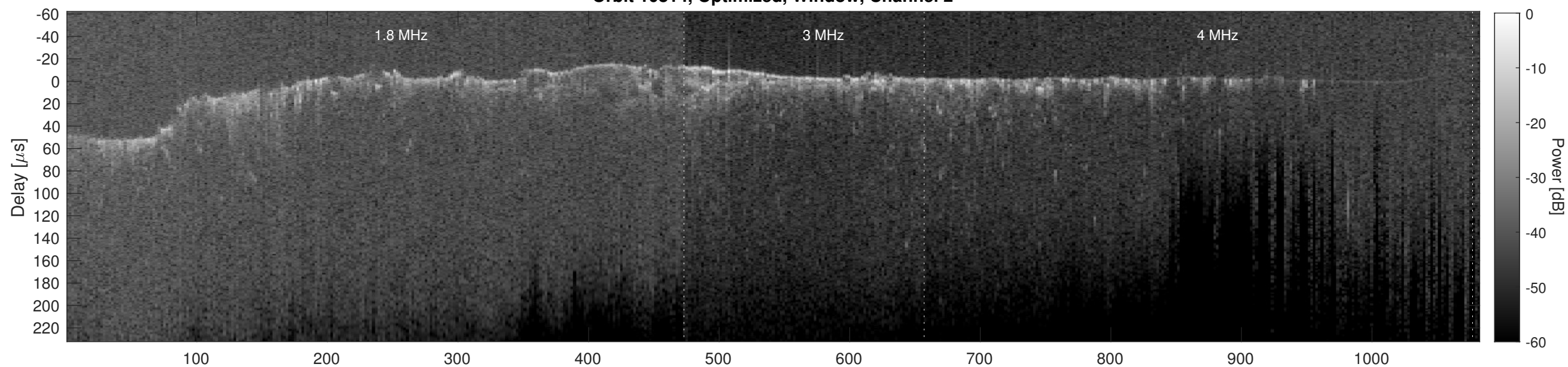
Orbit 10814, Cluttergram
