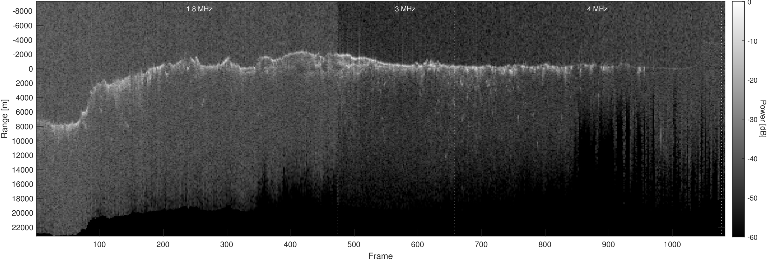
Orbit 10814, Optimized, Window, Depth-Corrected, Channel 2
