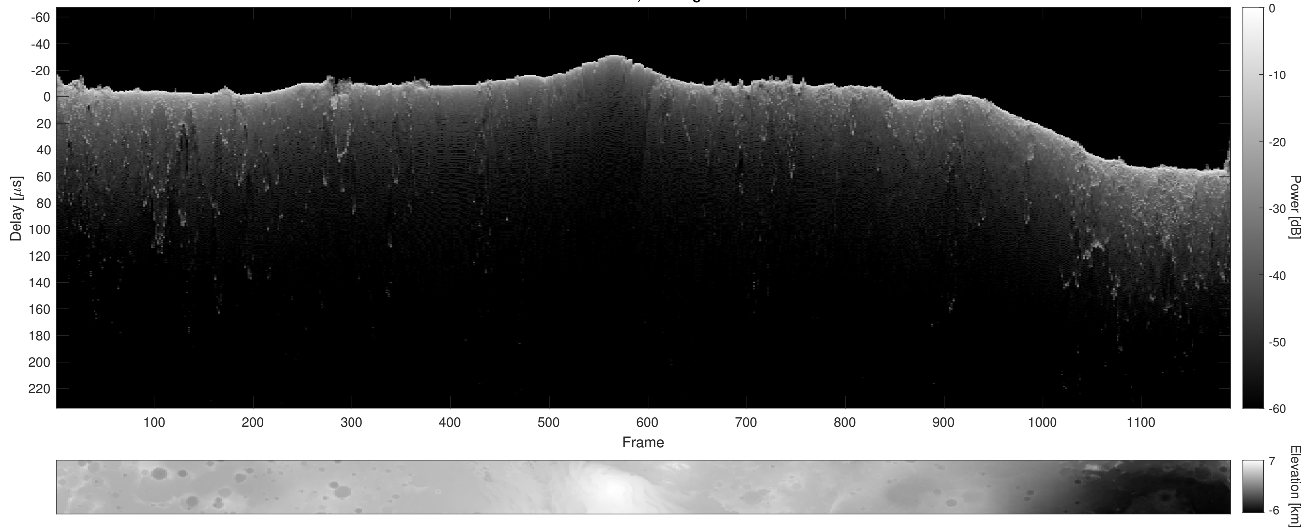
Orbit 10816, Cluttergram
