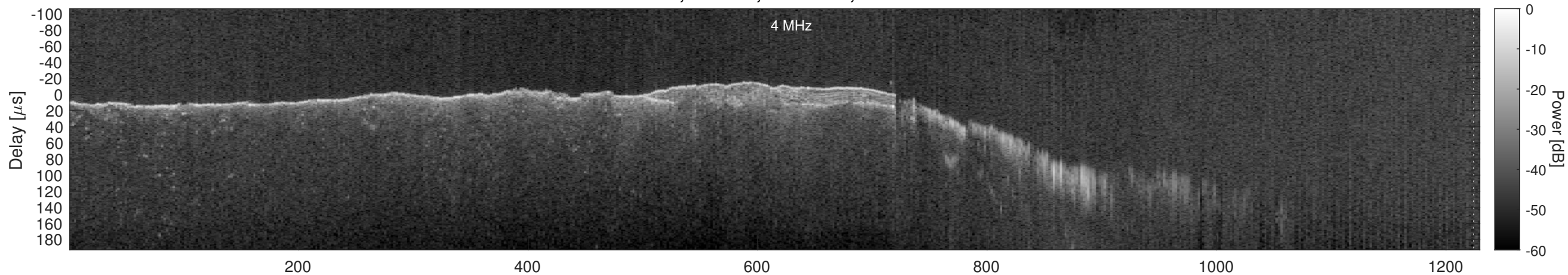
Orbit 10818, Window, Channel 2, Chapman
