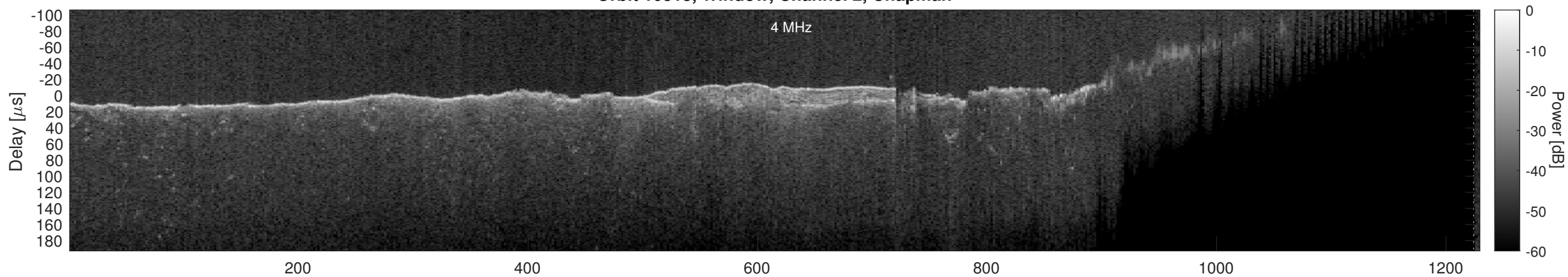
Orbit 10818, Window, Channel 2, Optimized
