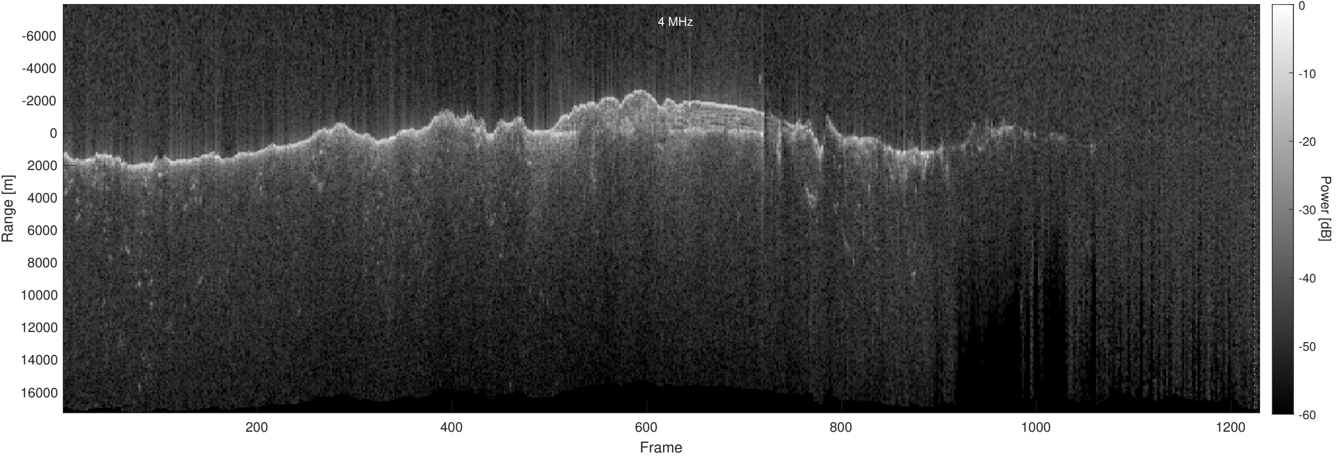
Orbit 10818, Optimized, No Window, Depth-Corrected, Channel 2
