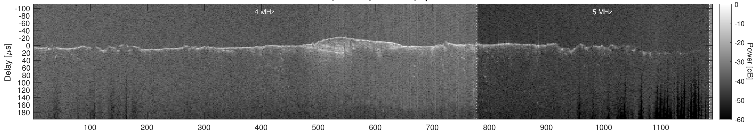
Orbit 10819, Cluttergram
