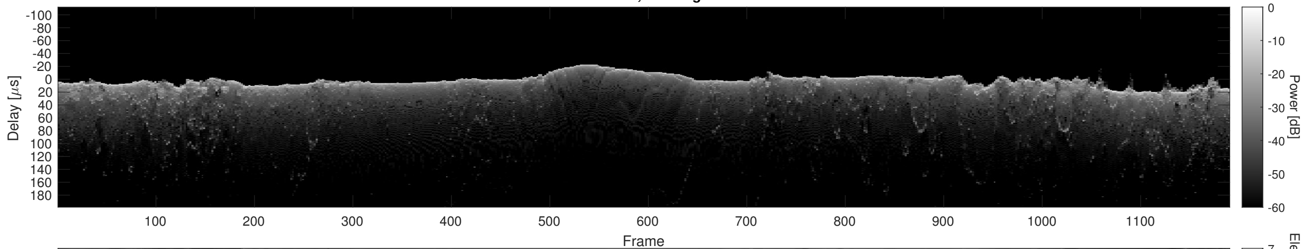
Orbit 10819, Cluttergram
