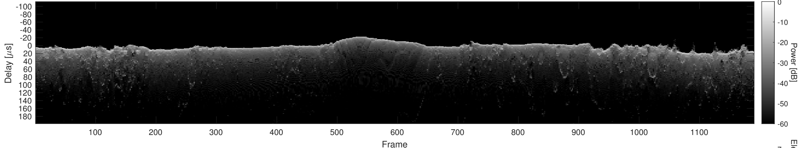
Orbit 10819, Cluttergram
