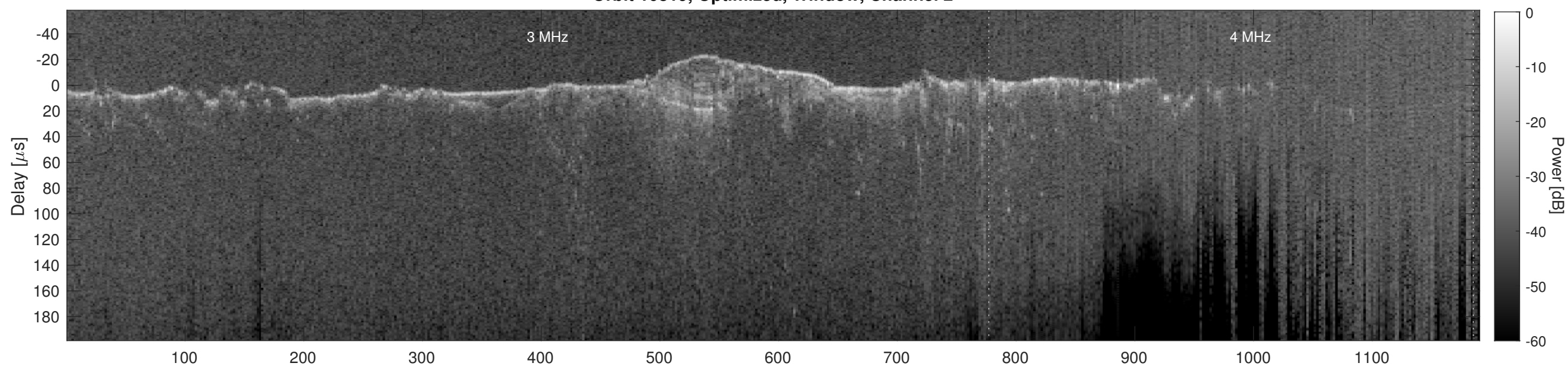
Orbit 10819, Cluttergram
