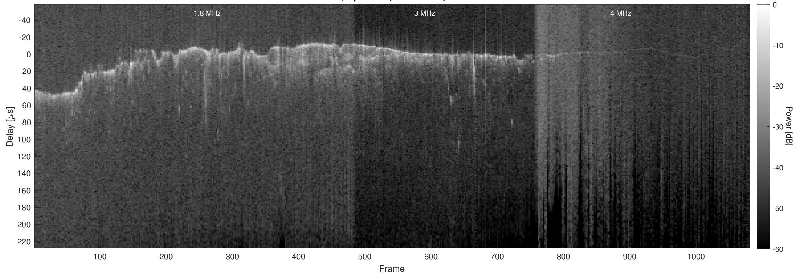
Orbit 10821, Optimized, No Window, Channel 2
