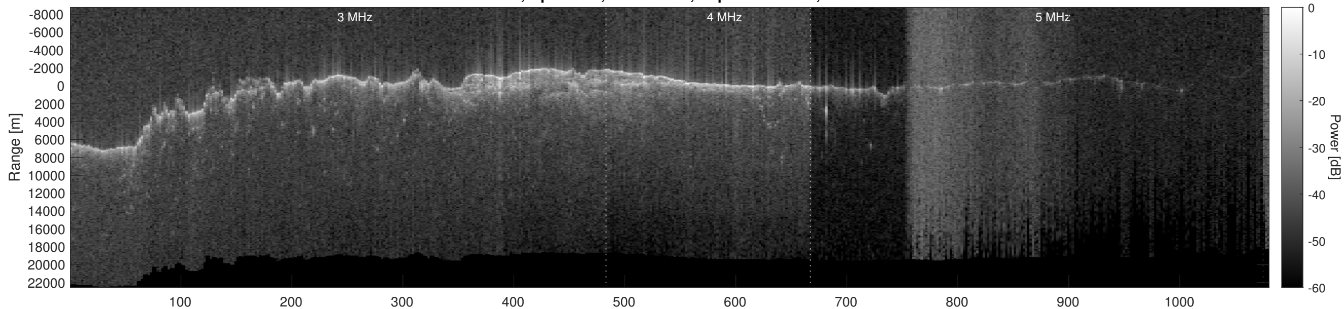
Orbit 10821, Optimized, No Window, Depth-Corrected, Channel 2
