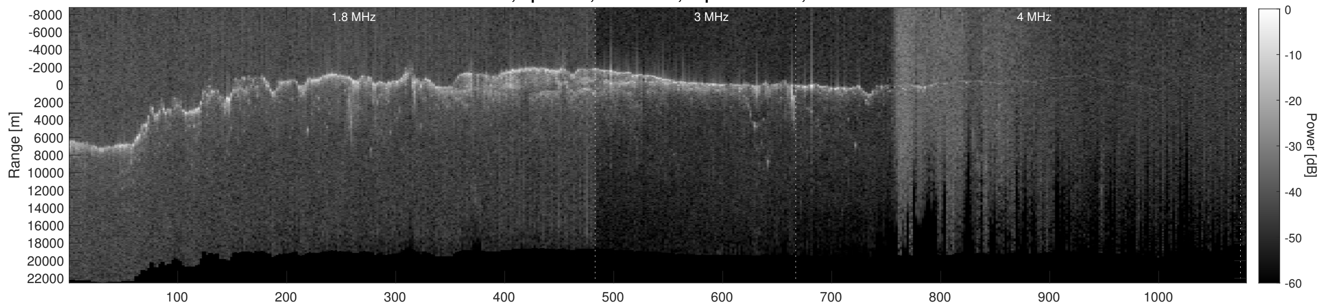
Orbit 10821, Depth-Corrected Cluttergram
