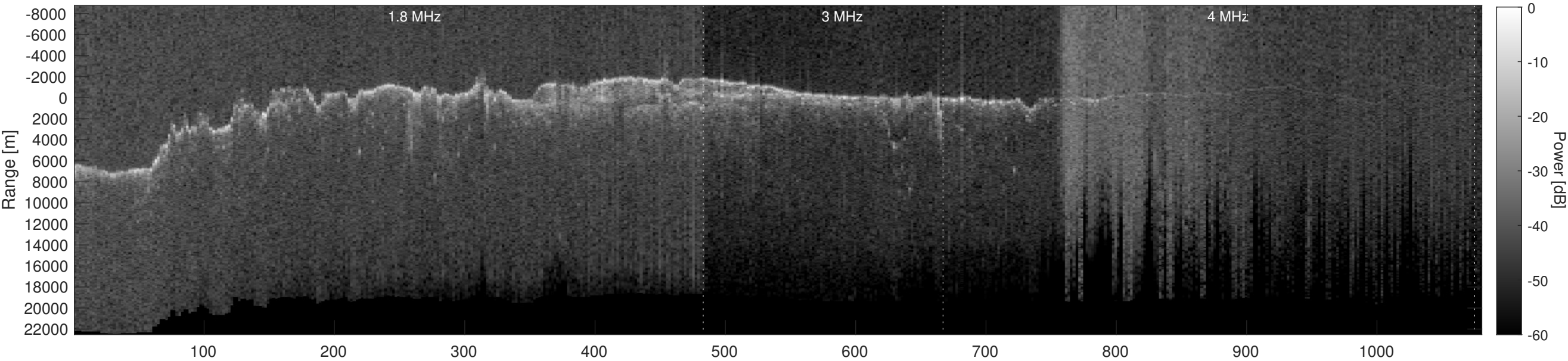
Orbit 10821, Depth-Corrected Cluttergram
