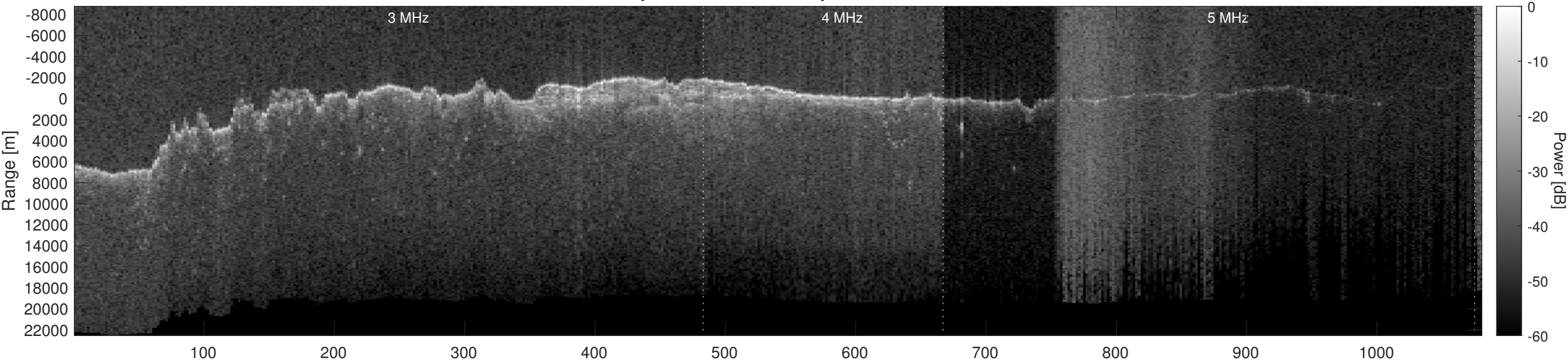
Orbit 10821, Optimized, Window, Depth-Corrected, Channel 2
