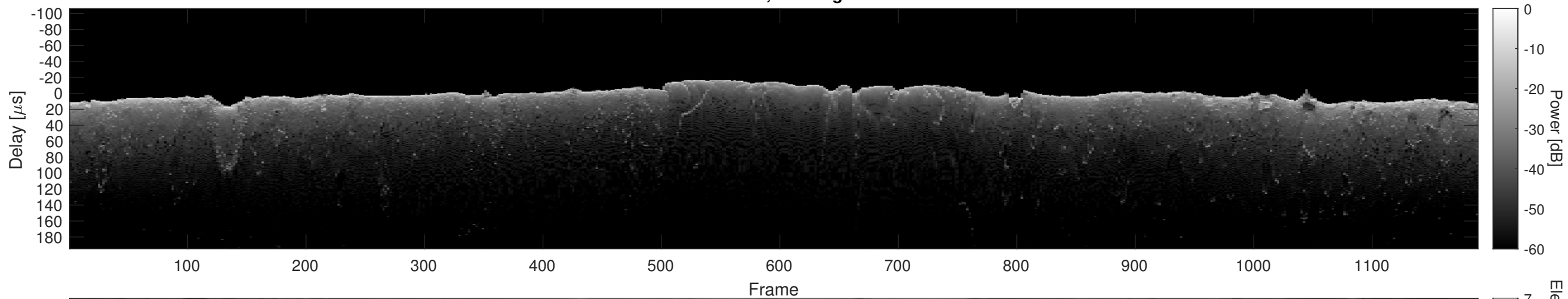
Orbit 10822, Cluttergram
