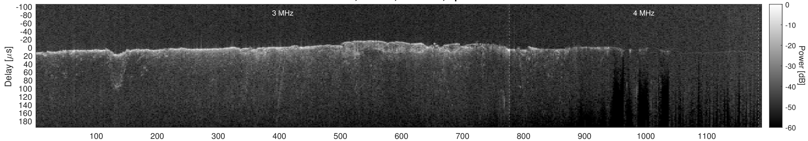
Orbit 10822, Cluttergram
