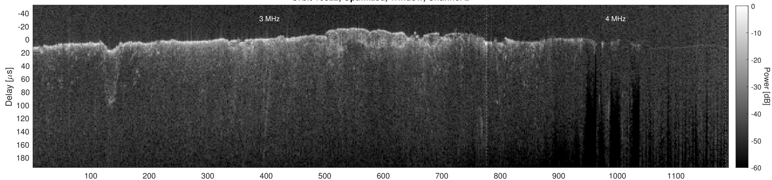
Orbit 10822, Cluttergram
