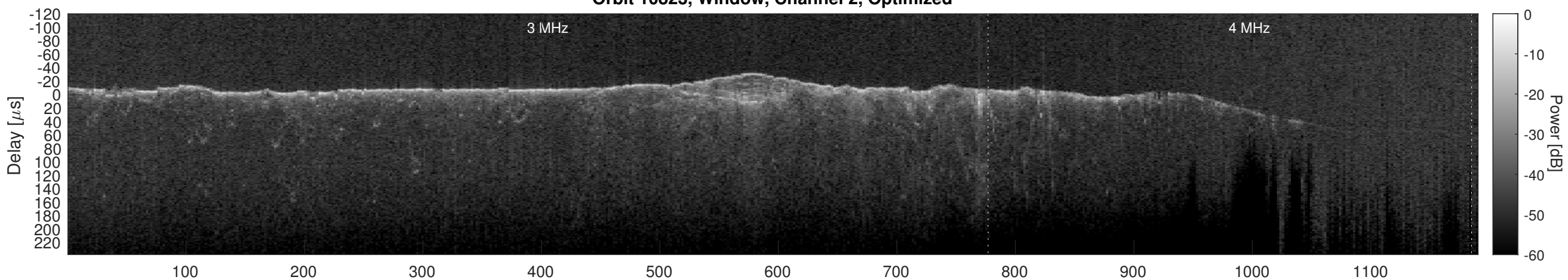
Orbit 10823, Cluttergram
