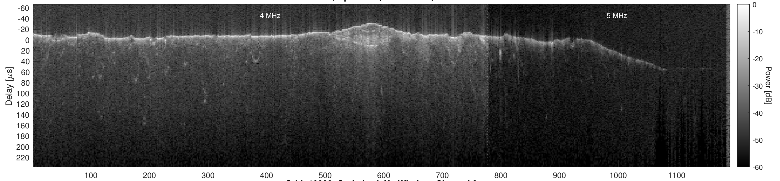
Orbit 10823, Optimized, No Window, Channel 2
