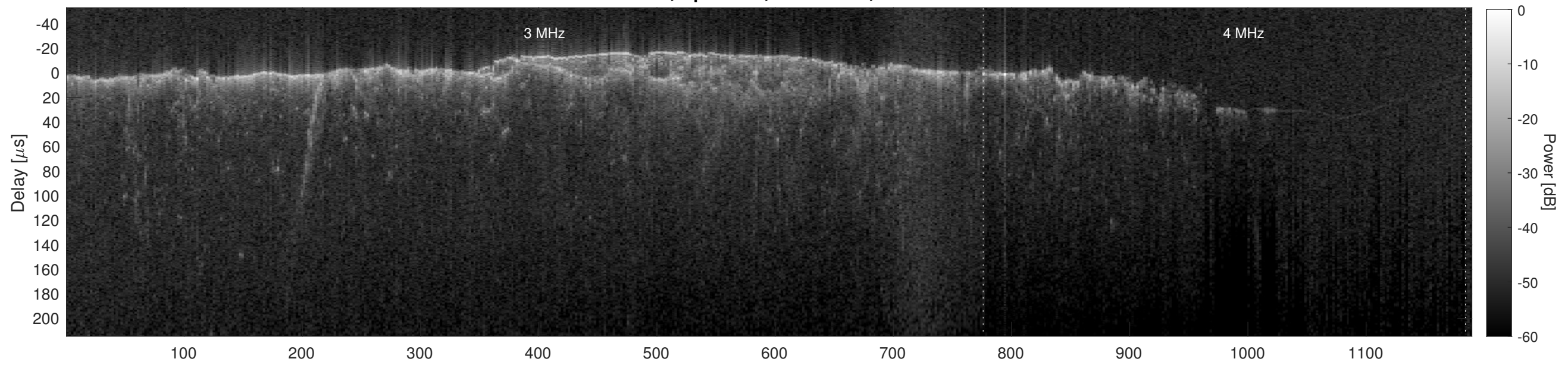
Orbit 10824, Cluttergram
