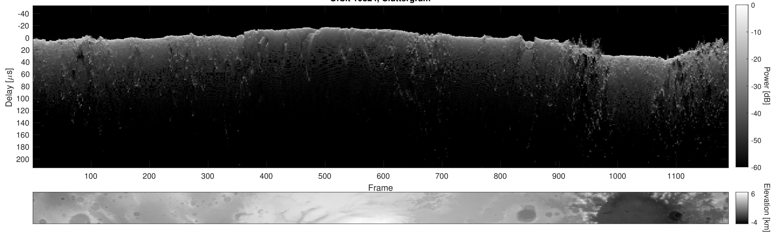
Orbit 10824, Cluttergram
