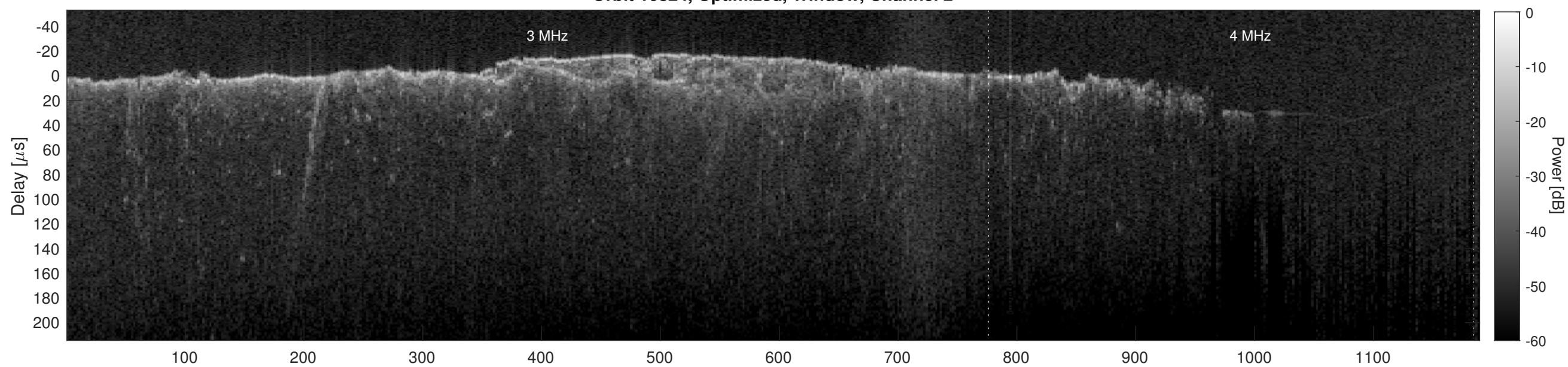
Orbit 10824, Cluttergram
