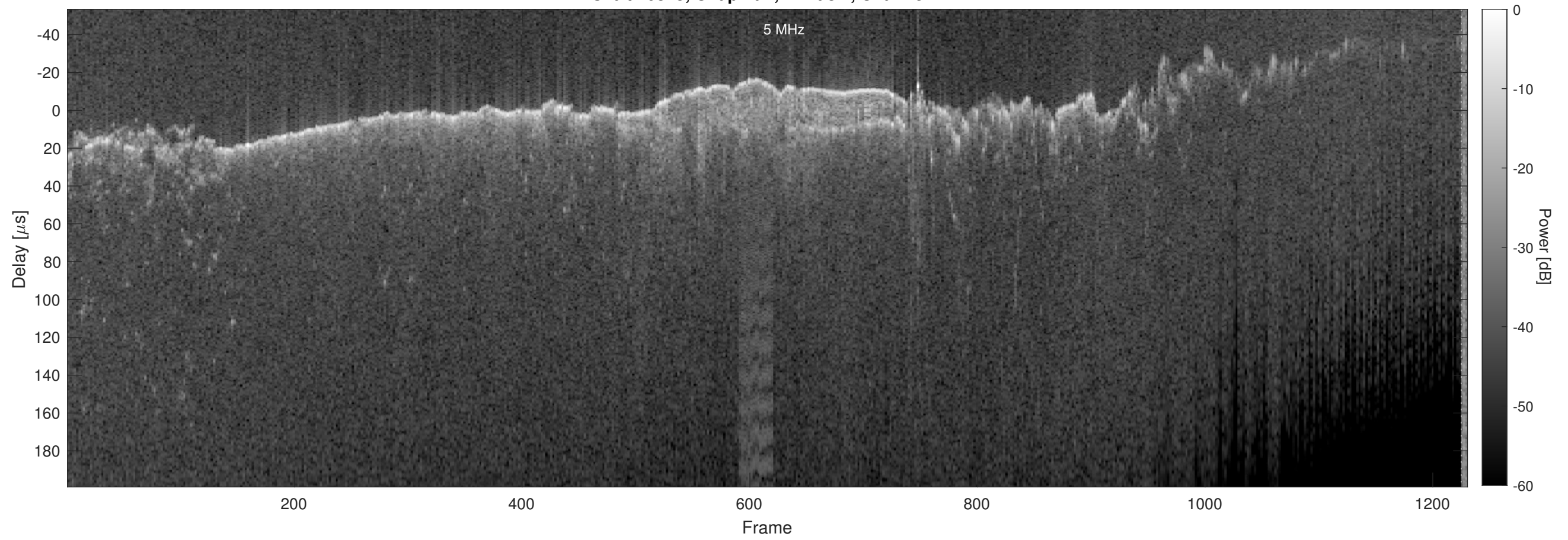
Orbit 10825, Chapman, Window, Channel 2
