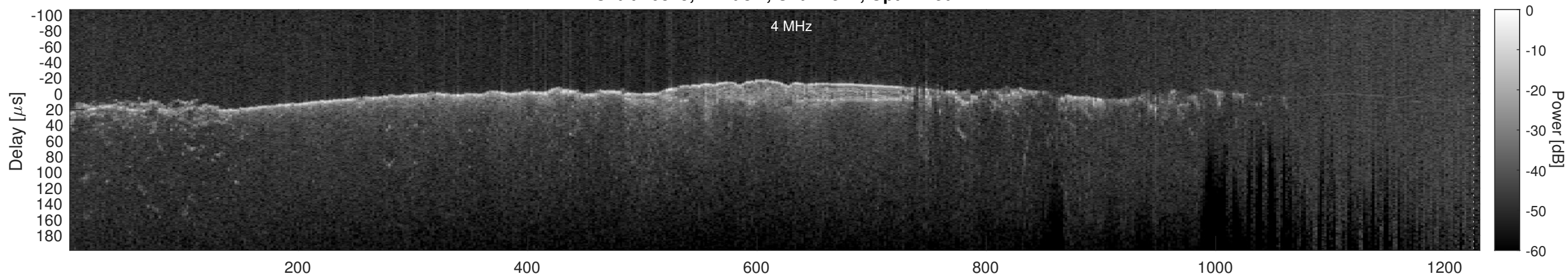
Orbit 10825, Cluttergram
