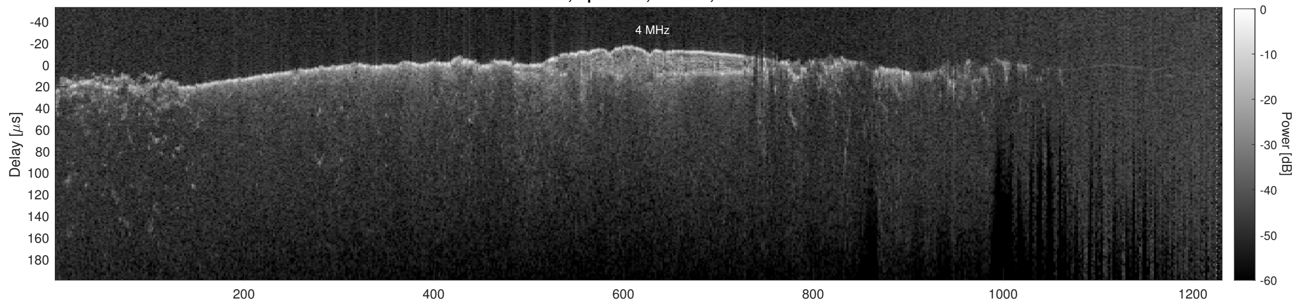
Orbit 10825, Cluttergram
