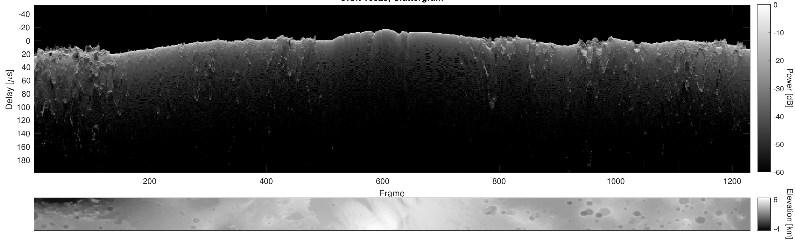
Orbit 10825, Cluttergram
