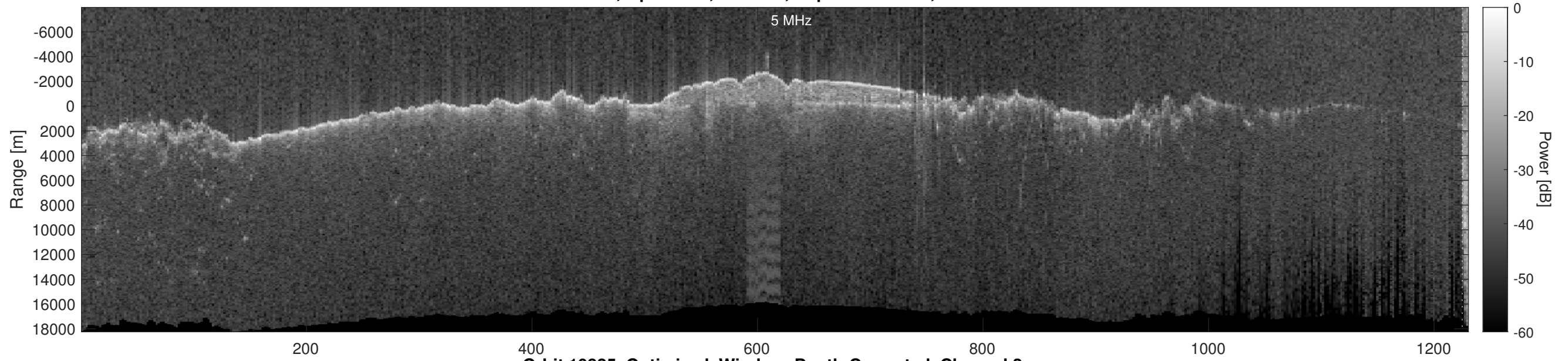
Orbit 10825, Optimized, Window, Depth-Corrected, Channel 2
