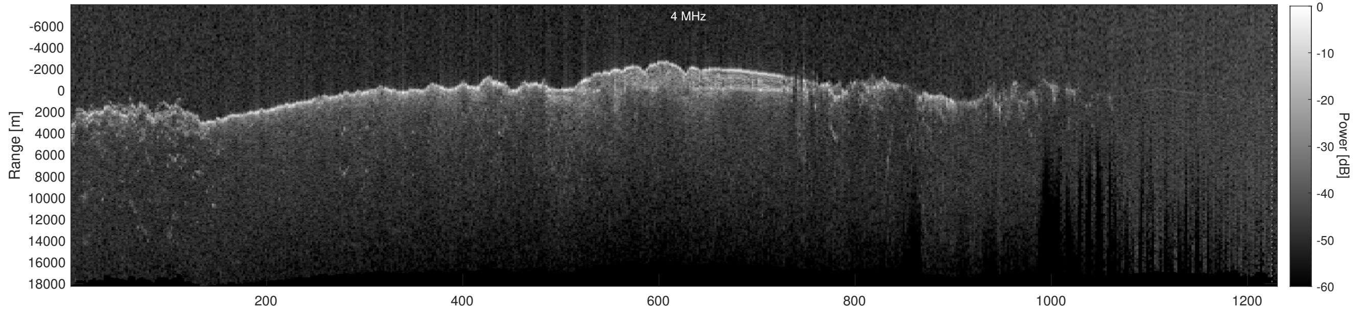
Orbit 10825, Depth-Corrected Cluttergram
