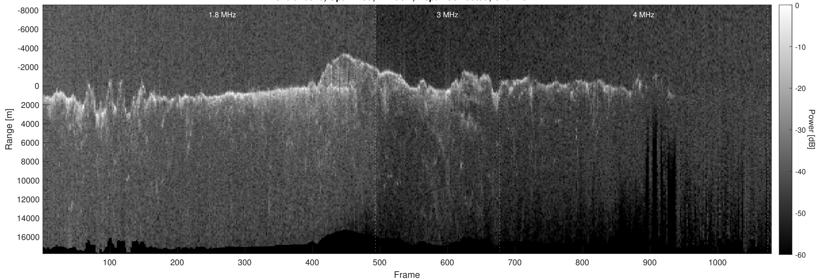
Orbit 10826, Optimized, Window, Depth-Corrected, Channel 2
