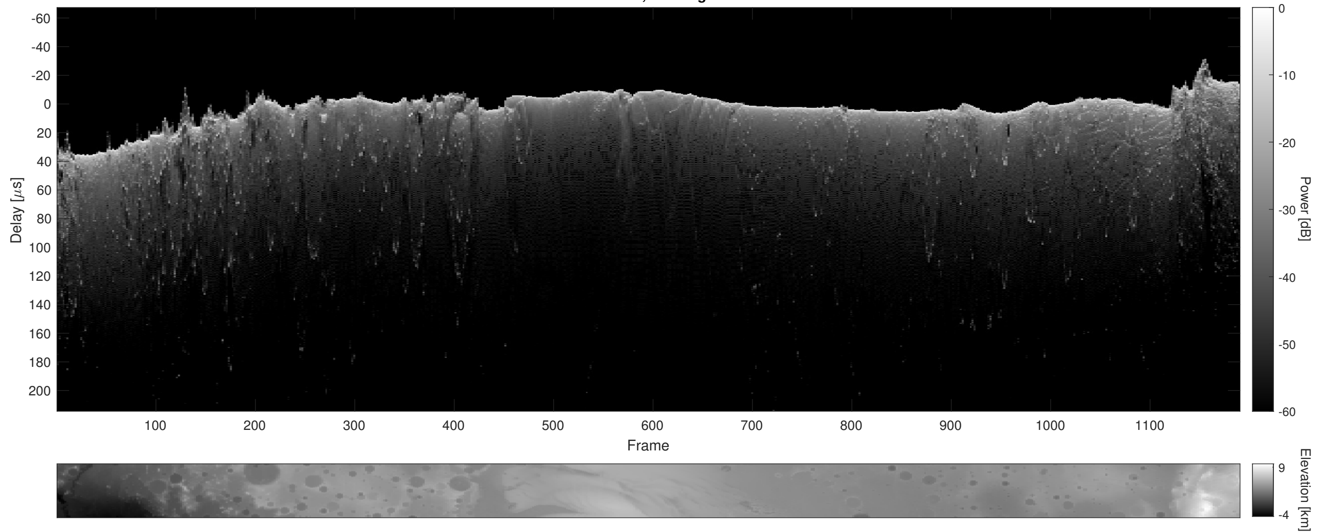
Orbit 10828, Cluttergram
