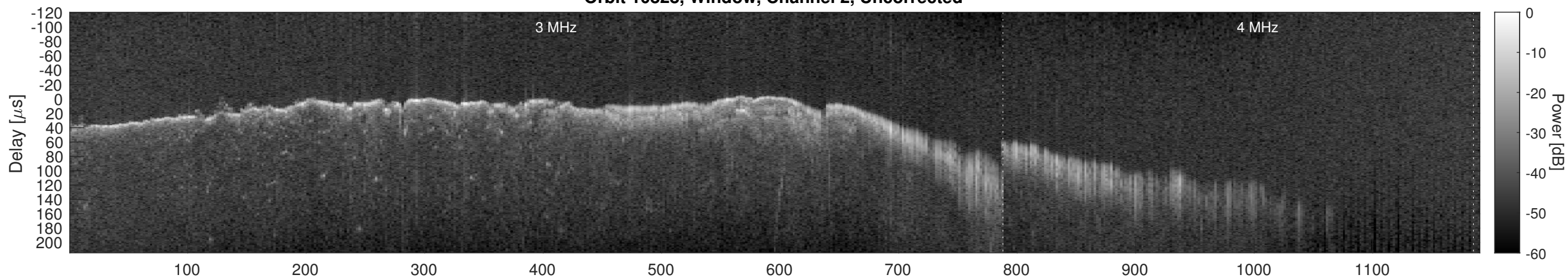
Orbit 10828, Window, Channel 2, Chapman
