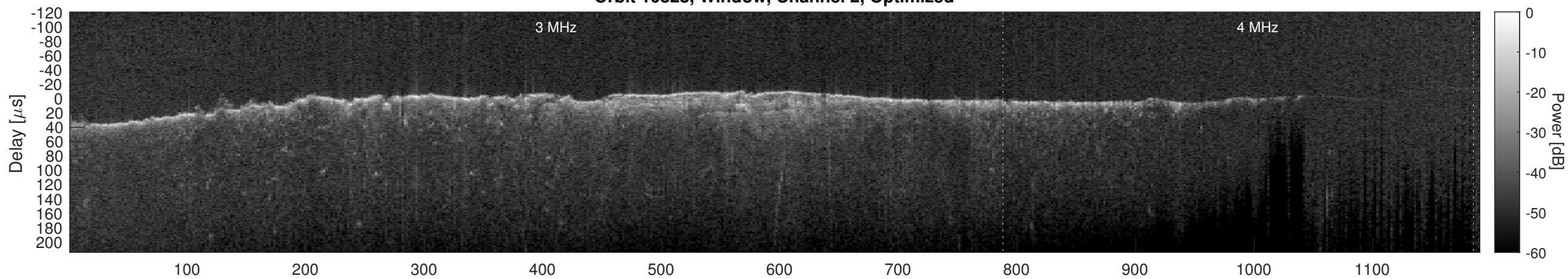
Orbit 10828, Cluttergram
