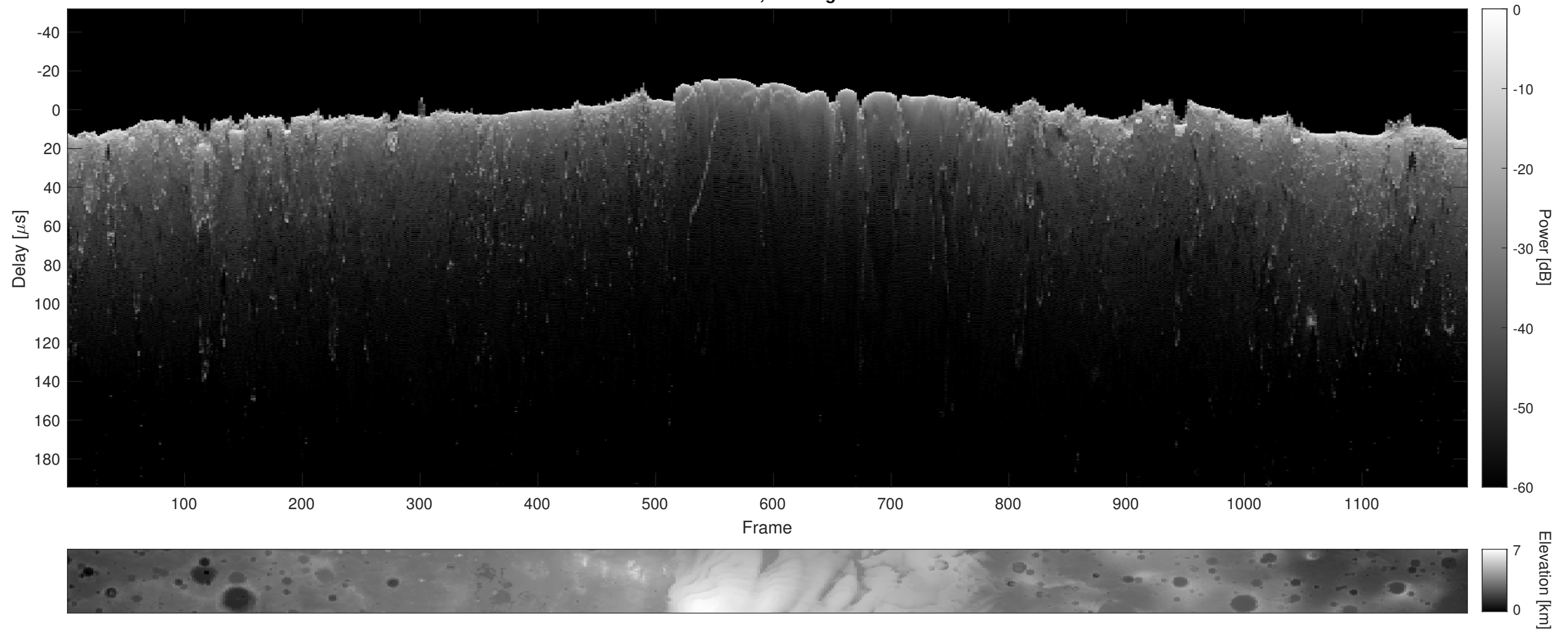
Orbit 10829, Cluttergram
