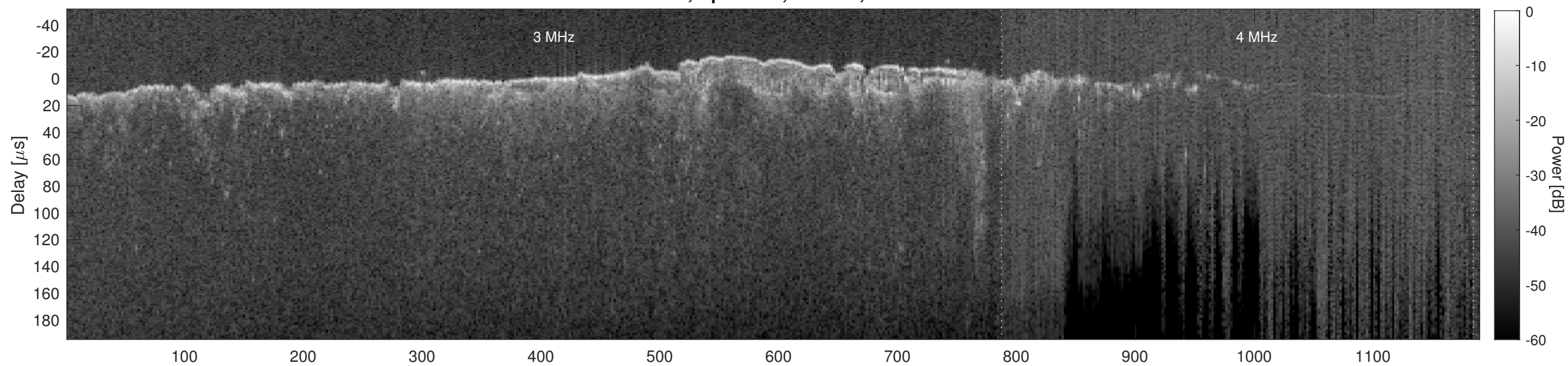
Orbit 10829, Cluttergram
